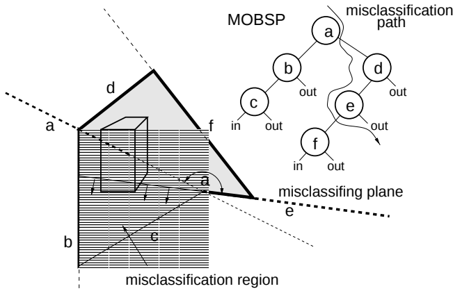
Figure 8. An example of disadvantageous configuration of occluders. The shadow planes of the MOBSP are shown by thin lines. The invisible polyhedra intersecting both the shadow plane a and the marked region is said to be partially visible.
