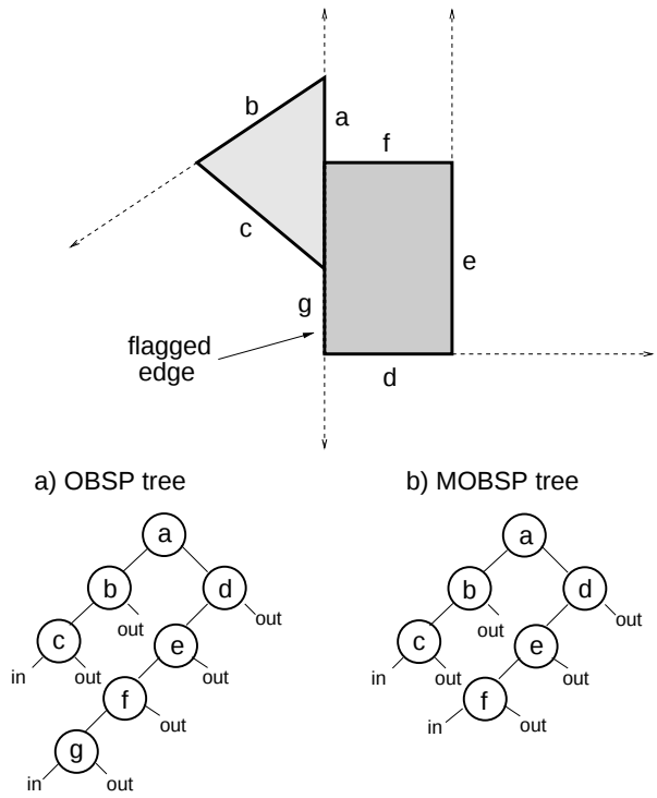
Figure 7. The difference between the OBSP and the MOBSP. Both trees are constructed with respect to the same occluders. The occluders are shown as seen from the view-point. Node g is not present in the MOBSP, since the corresponding occluder-edge was flagged.
