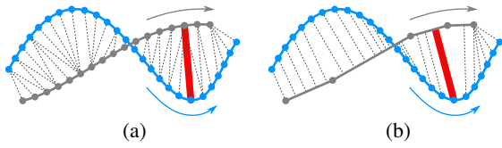
Figure 7: Discrete Fréchet distance. The minimum length of the line connecting ordered sets of point samples (a). Since we store the resolved paths in the simplified form, we compute the Fréchet distance between an ordered set of points and an ordered set of line segments (b) rather than between two point sets.
