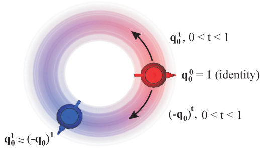
Fig. 22. Dual quaternions inherit the antipodality of classical quaternions. In this example, transformation of the teapot by \mathbf{q}_0^t for t \in [0, 1] produces a counterclockwise rotation (longer trajectory), while transformation by (-\mathbf{q}_0)^t leads to a clockwise one (shorter trajectory).
