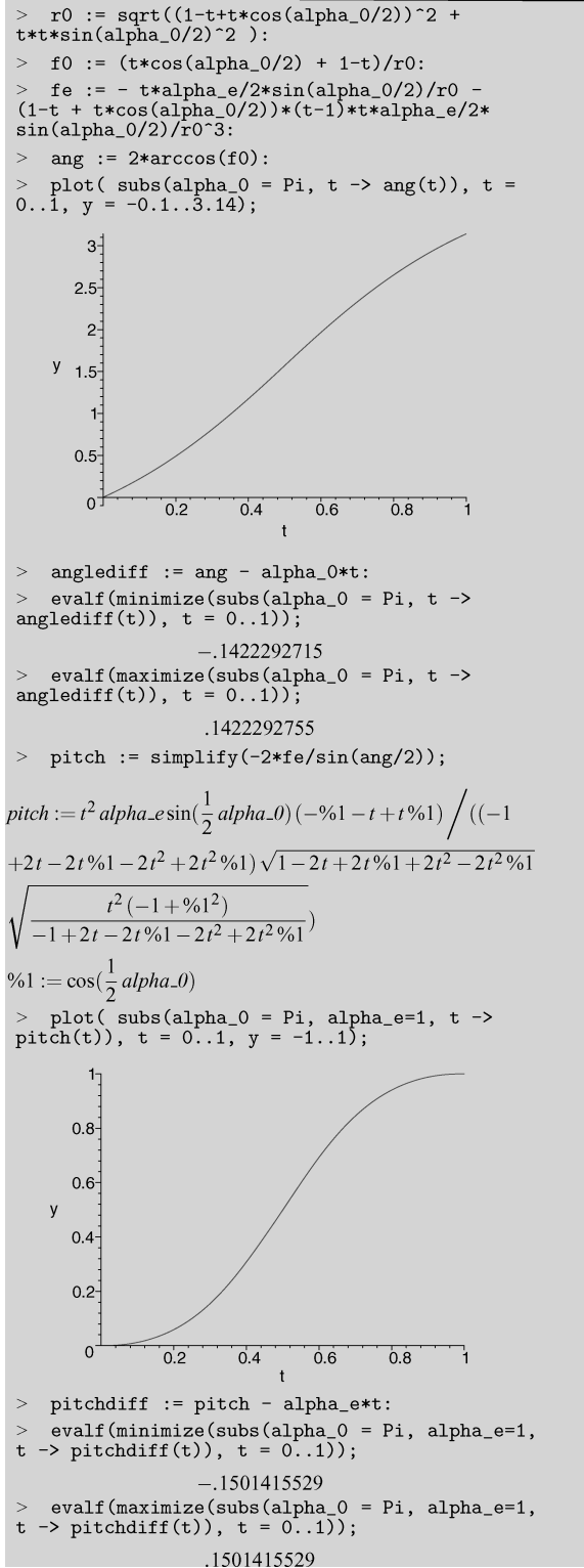
Fig. 23. Upper bound of the difference between ScLERP and DLB for n = 2 , computed using Maple.
