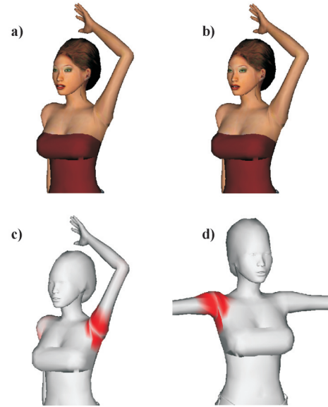
Fig. 25. Comparison of DLB and DIB applied in skinning. The difference between DLB (a) and DIB (b) is imperceptible even for large joint rotations and therefore we visualize it using color in (c) and (d).
