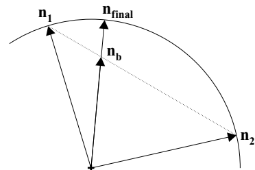
Fig. 3. Standard normal blending trick: vectors \mathbf{n}_1 and \mathbf{n}_2 are first blended linearly giving \mathbf{n}_b and then re-normalized, giving \mathbf{n}_{final} .
