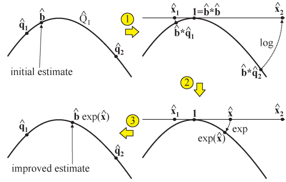
Fig. 24. Illustration of one iteration of the DIB algorithm.
