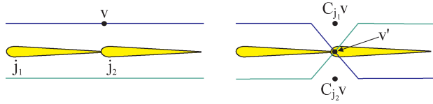
Fig. 4. A typical “candy-wrapper” artifact of linear blend skinning. On the left is a reference pose and on the right an animated one.
