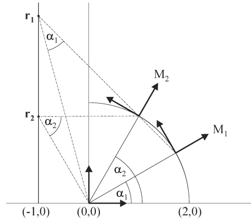
Fig. 9. Interpolation between transformations M_1 and M_2 \in SE(2) with rotation centers \mathbf{r}_1 and \mathbf{r}_2 . Note that the angle of rotation is the same with respect to any center.
