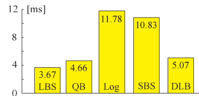
Fig. 18. Average CPU performance for skin deformation of the human model in milliseconds (Pentium 4, 3.4 GHz): LBS—linear blend skinning, QB—direct quaternion blending, Log—log-matrix blending, SBS—spherical blend skinning, DLB—dual quaternion linear blending (pre-computed antipodality).
