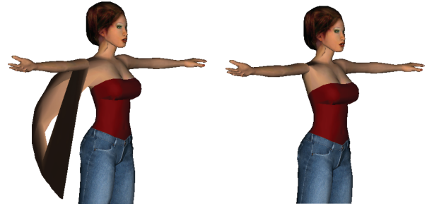
Fig. 6. Artifacts produced by blending rotations with respect to the origin (left) are even worse than those of linear blend skinning (right).
