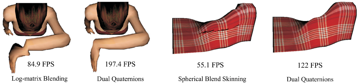
Fig. 1. A comparison of dual quaternion skinning with previous methods: log-matrix blending [Cordier and Magnenat-Thalmann 2005] and spherical blend skinning [Kavan and Žára 2005]. The proposed approach not only eliminates artifacts, but is also much easier to implement and more than twice as fast.
