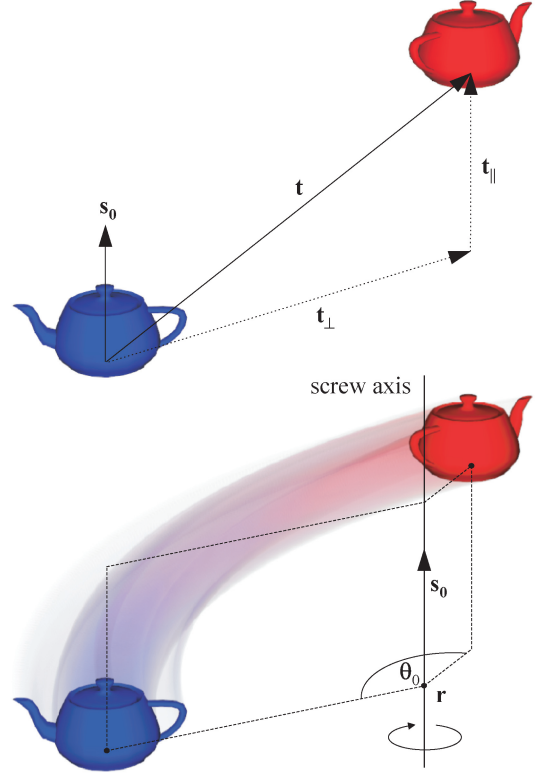
Fig. 21. Conversion of a rotation about axis \mathbf{s}_0 , \|\mathbf{s}_0\| = 1 , followed by translation \mathbf{t} (top) to the corresponding screw (bottom).
