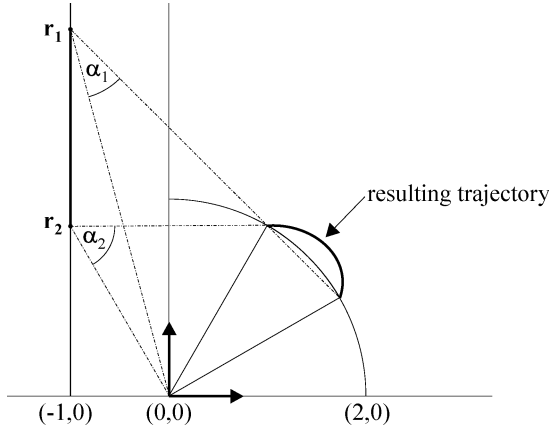
Fig. 10. Trajectory resulting from linear interpolation of rotation centers.
