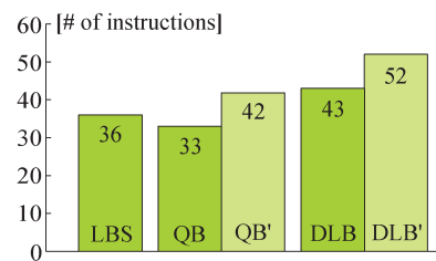
Fig. 19. Number of vertex shader instructions: LBS—linear blend skinning, QB—direct quaternion blending (pre-computed antipodality), DLB—dual quaternion linear blending (pre-computed antipodality), QB' and DLB'—same as before but with antipodality resolved in the vertex shader.
