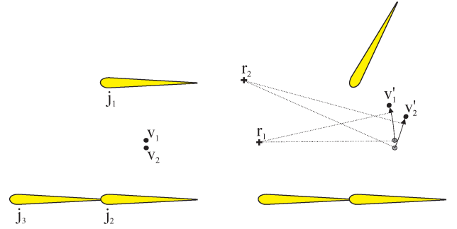
Fig. 8. Problem with rotation centers in spherical blend skinning. On the left is a reference pose and on the right an animated one.
