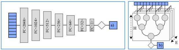
Fig. 11. ICTreeF Model (left) : The feature-based realism predictor consists of a shrinking sequence of fully connected layers, each followed by a ReLU activation. Finally, the last layer utilizes a Leaky ReLU activation and outputs the predicted score value (a). Feature Importance Model (right) : analysis is performed by fitting a Random Forest Regressor ensemble, using MSE criterion to train against the ground-truth tree scores (b).
