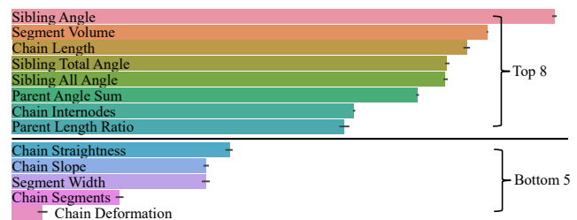
Fig. 15. Feature Importance: eight most important features (top) and five least important (bottom) are displayed. The x -axis is logarithmic and contains importance scores retrieved in feature analysis (Sect. 6.3).
