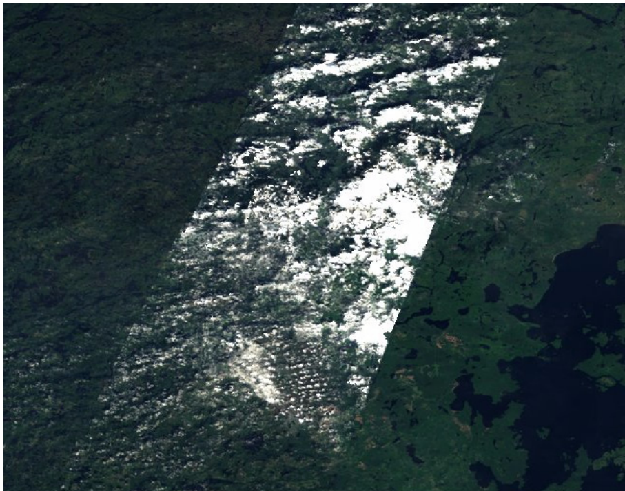
Figure 3.16: Example of more prominent cloud coverage in sentinel dataset.
