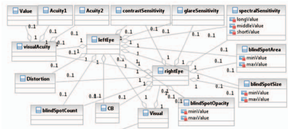
Figure 2.2: VUMS – Visual variables – UML class diagram, from [18].
